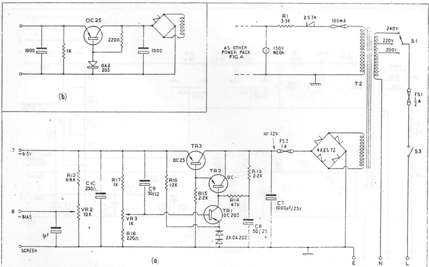
Fig. 3. The main circuit (a) shows a sophisticated transistorised stabilising arrangement for the DC heater supply, while the insert (b) is a simpler but less effective circuit.
