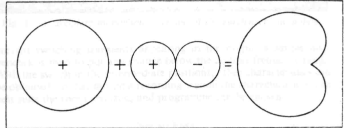
Fig. 3. Omni-directional plus figure-of-eight produces a cardioid
