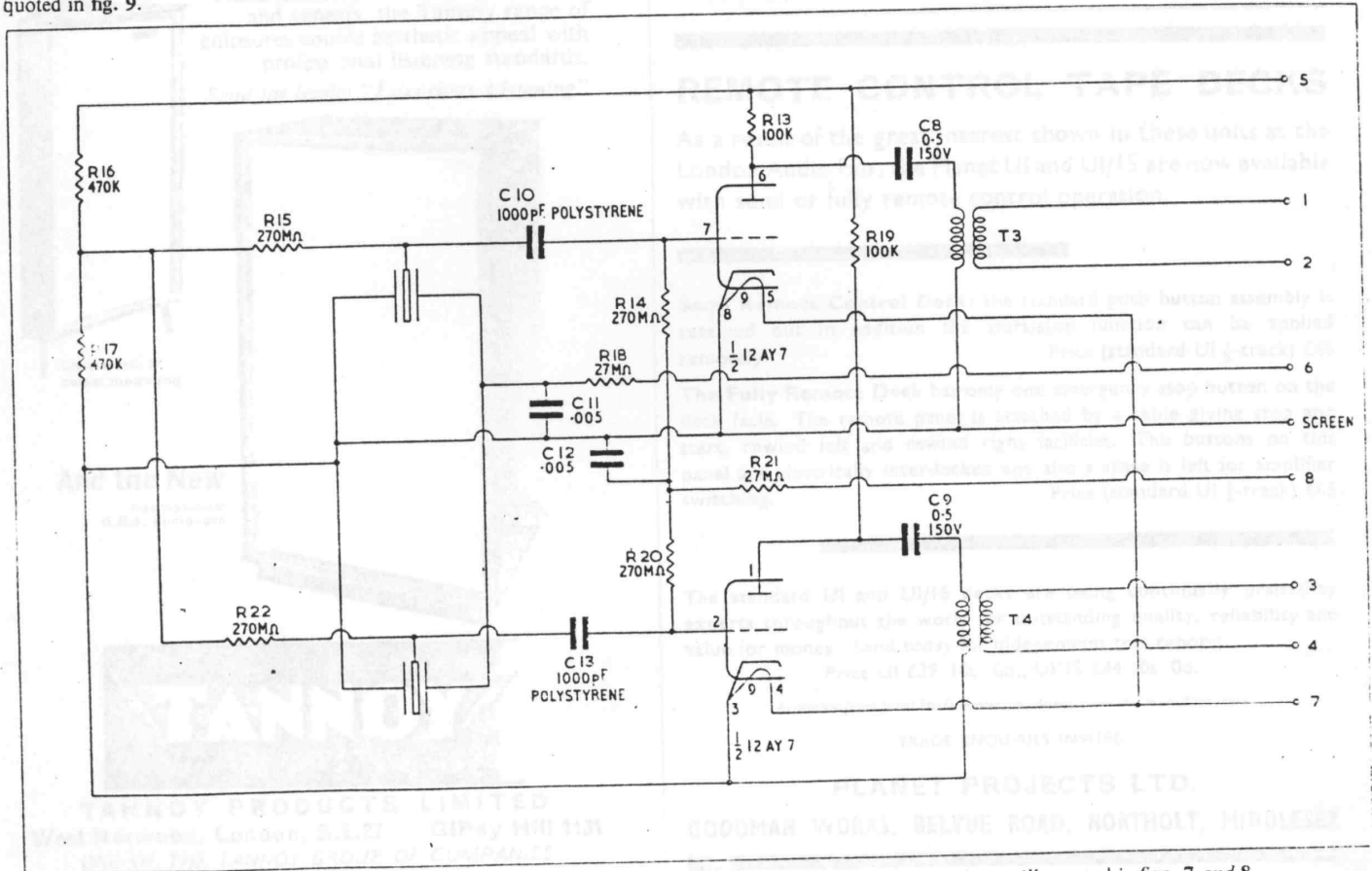
Fig. 5. Head pre-amplifier for the stereo microphone. This is all mounted beneath the capsules as illustrated in figs. 7 and 8
