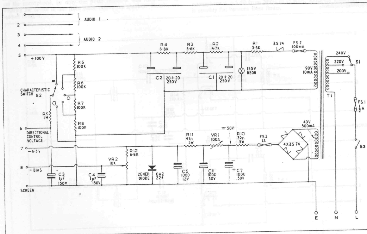
Fig. 4. The power supply circuit actually used in the prototype. This is housed in the control box shown in fig. 6
