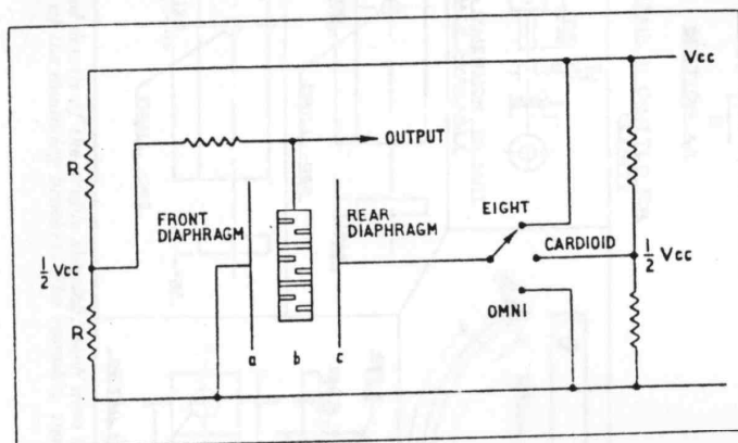
Fig. 6. Electrical circuit for changing the directional characteristics
